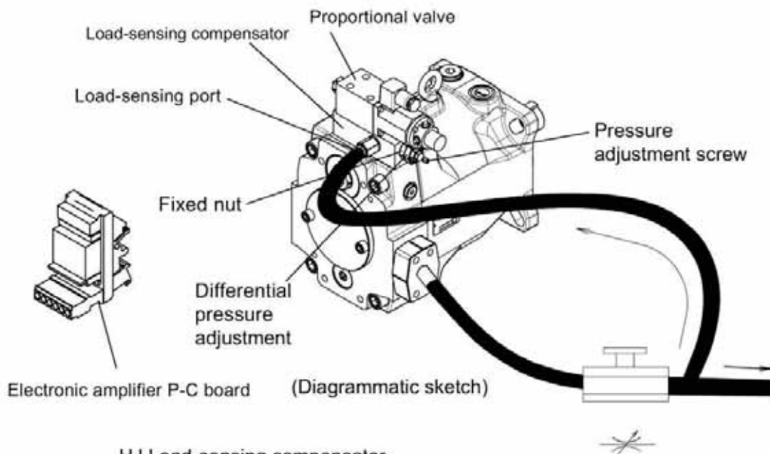
HJ Load-sensing compensator + Proportional pressure valve
