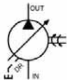
PV270 (Body 5)
